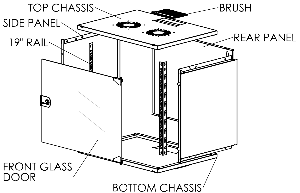
Exploded view
