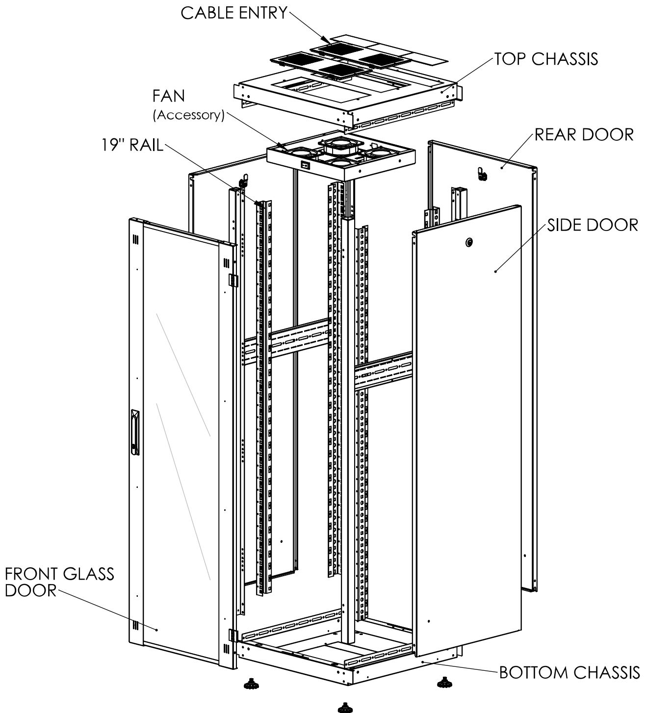
Exploded view
