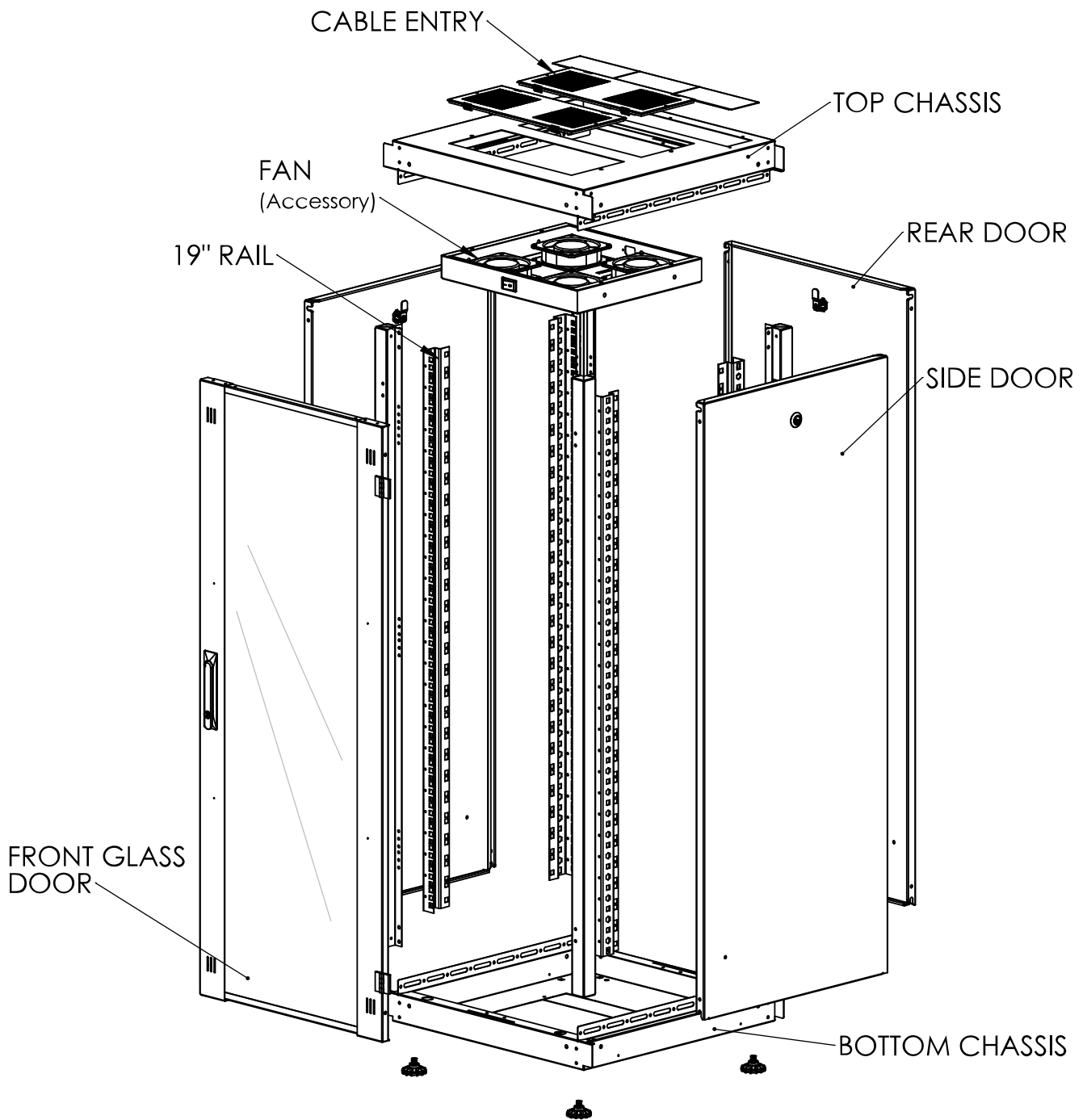
Exploded view
