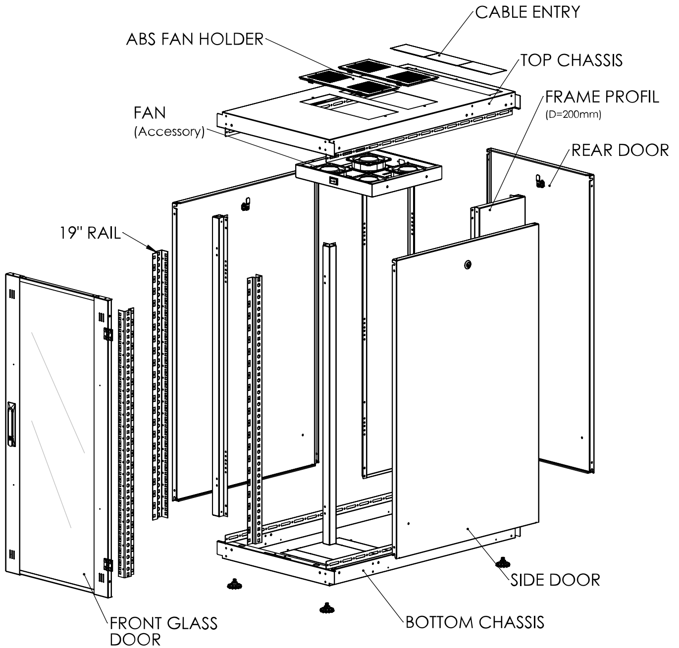
Exploded view
